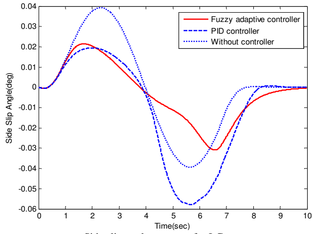
Fig21. Side slip angle response for LC maneuvre
