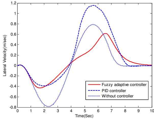
Fig22. Lateral velocity response for LC maneuvre
