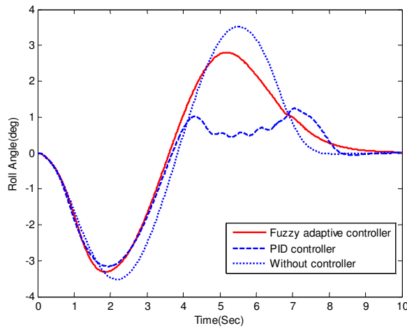
Fig23. Roll angle response for LC maneuvre
